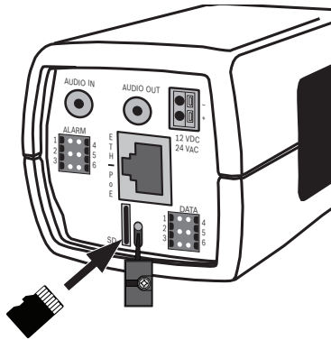
Figure 5.8 Inserting a microSD card
